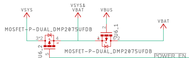
Vbat charge protection and power switch FET switches
