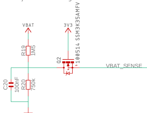
Battery sense voltage divisor
