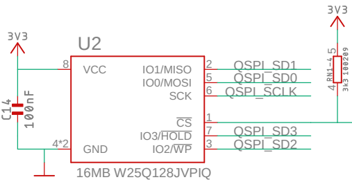
Flash memory
